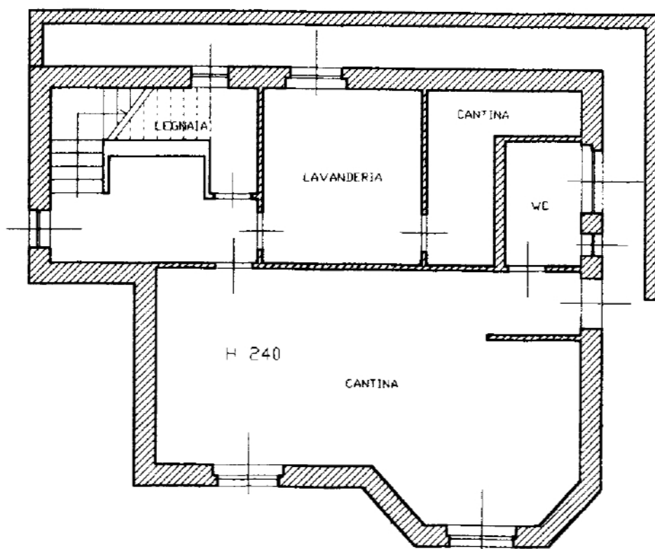
PIANO INTERRATO
