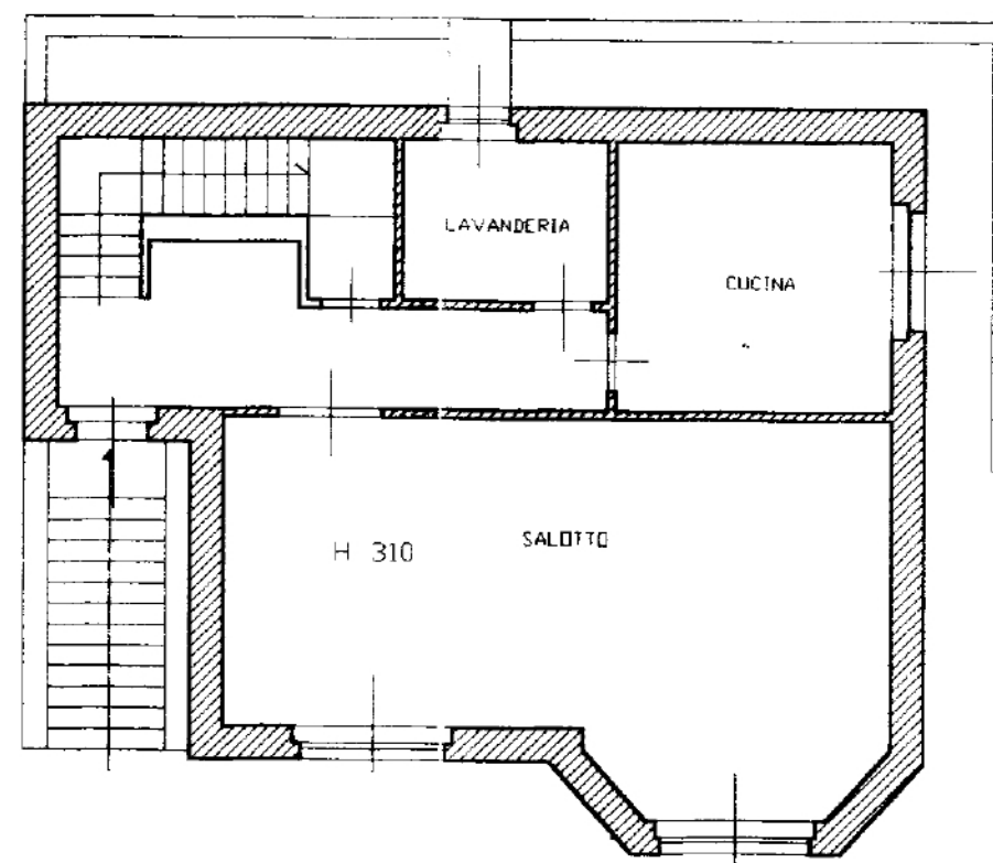
PIANO TERRA
