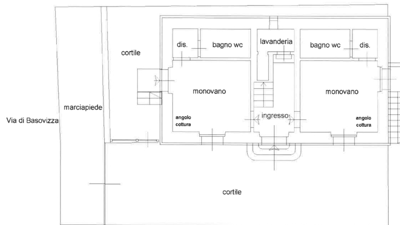
Piano terra
